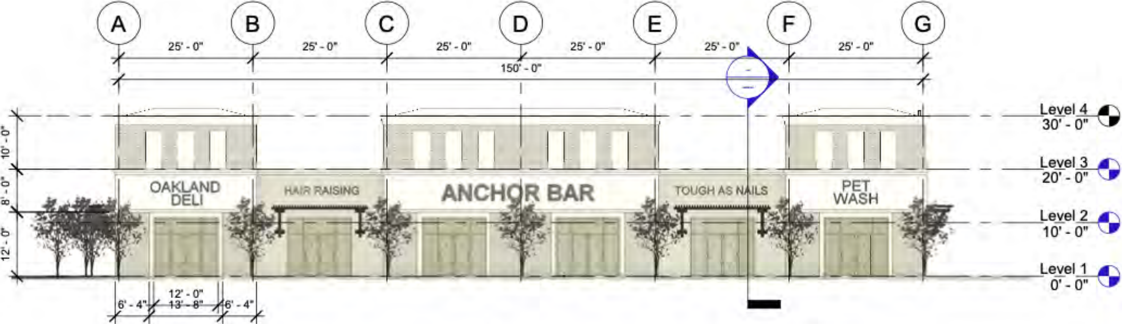
① West 1/16" = 1'-0"
